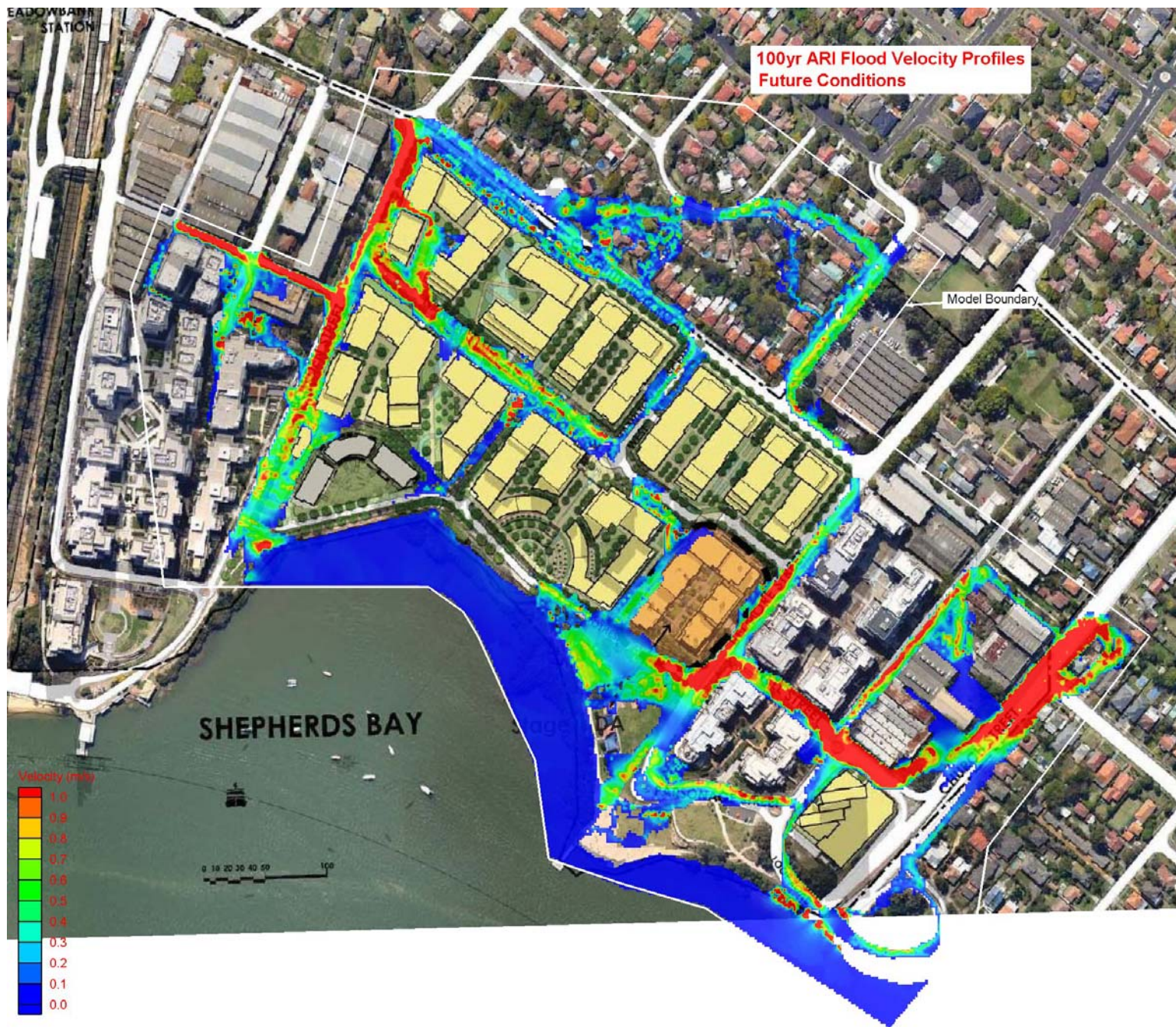
Figure 18 100 yr ARI Flood Velocities – Future Conditions
