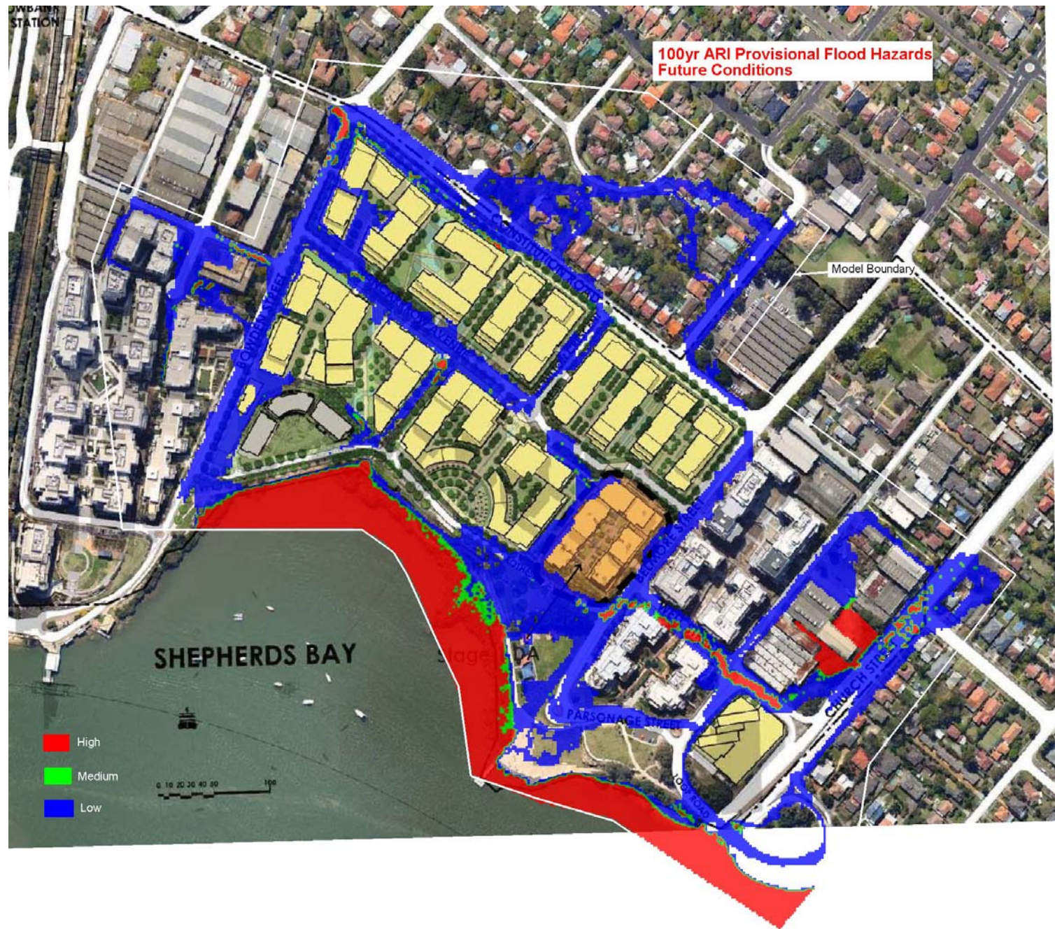
Figure 20 100 yr ARI Flood Hazard – Future Conditions
