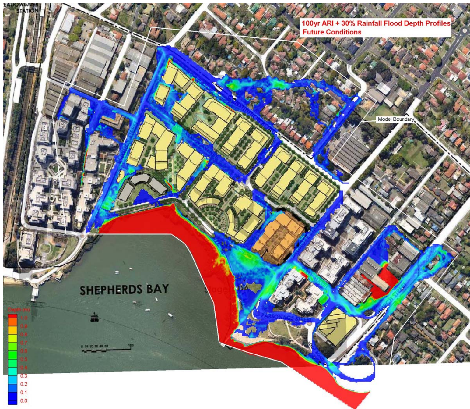
Figure 25 100 yr ARI Flood Levels – Future Conditions + 30% Increase in Rainfall
