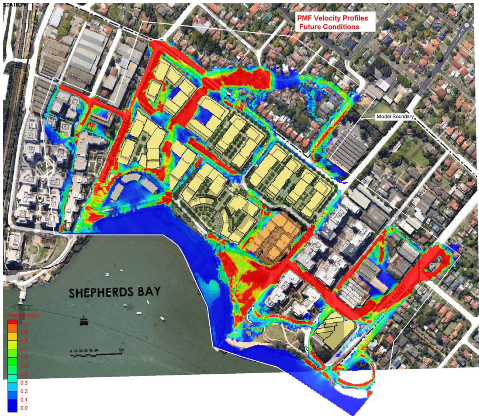
Figure 22 PMF Flood Velocities – Future Conditions
