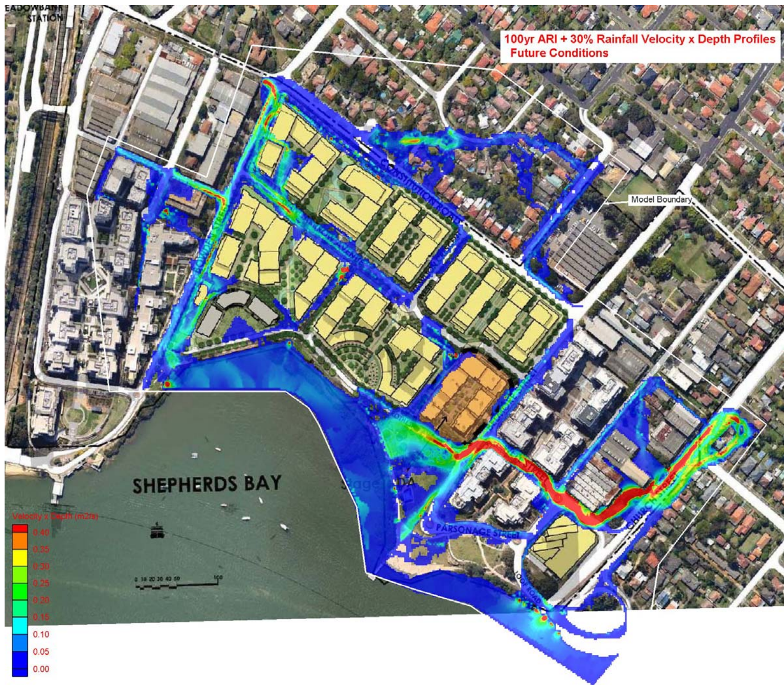
Figure 27 100 yr ARI Flood Velocity x Depth – Future Conditions + 30% Increase in Rainfall
