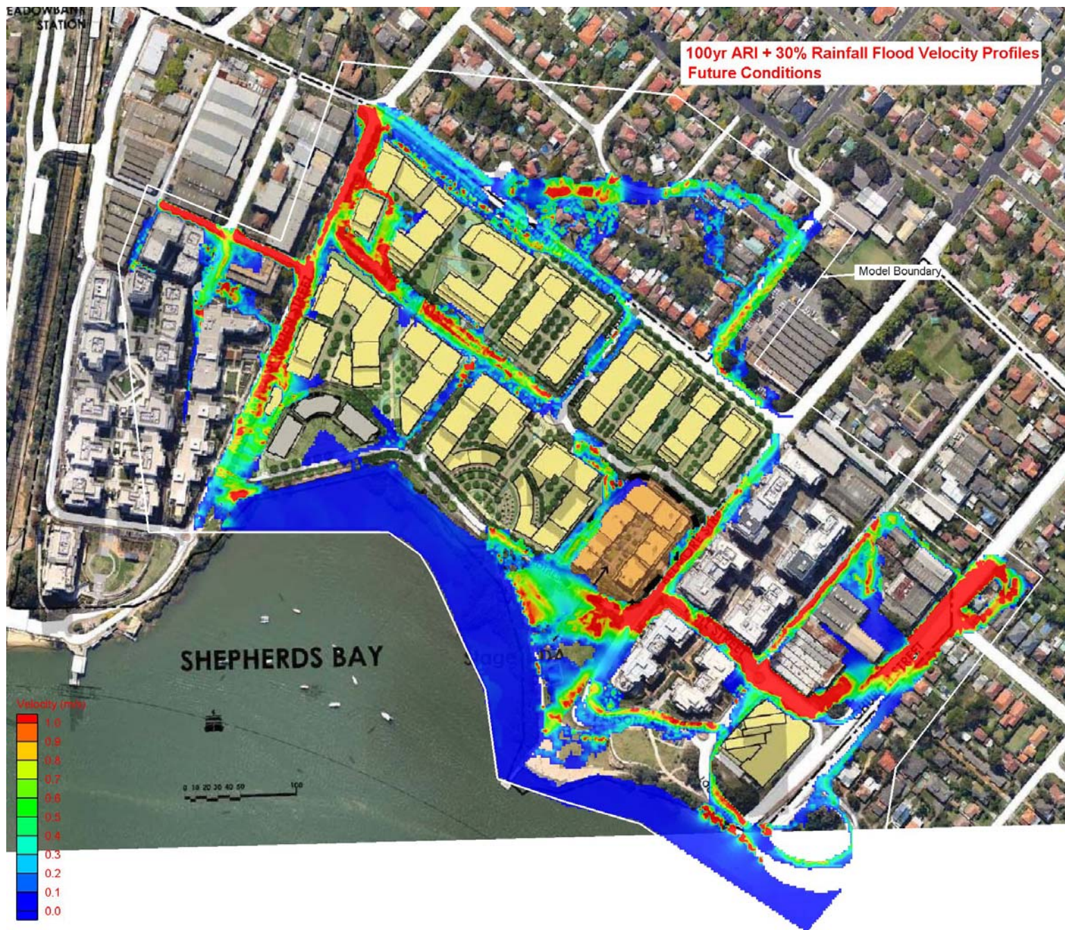
Figure 26 100 yr ARI Flood Velocities – Future Conditions + 30% Increase in Rainfall
