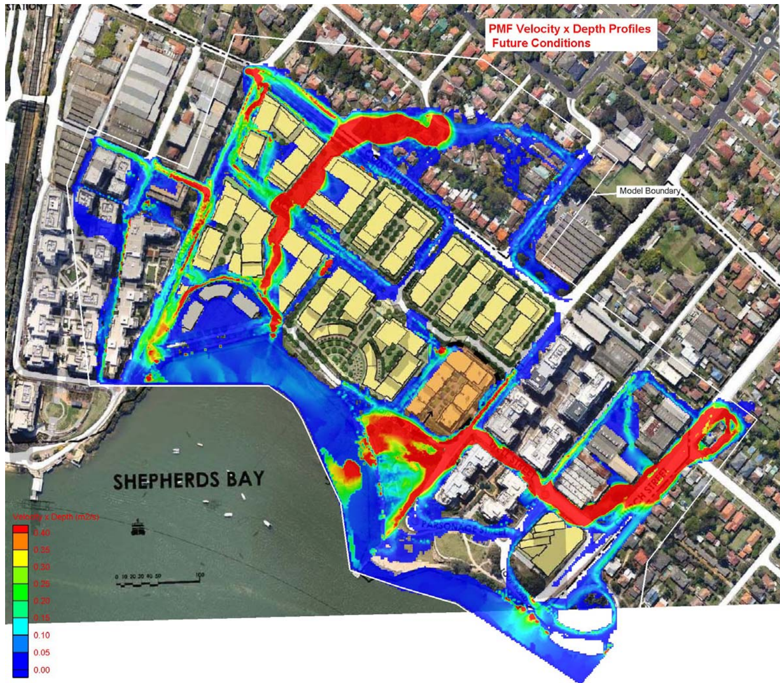
Figure 23 PMF Flood Velocity x Depth – Future Conditions
