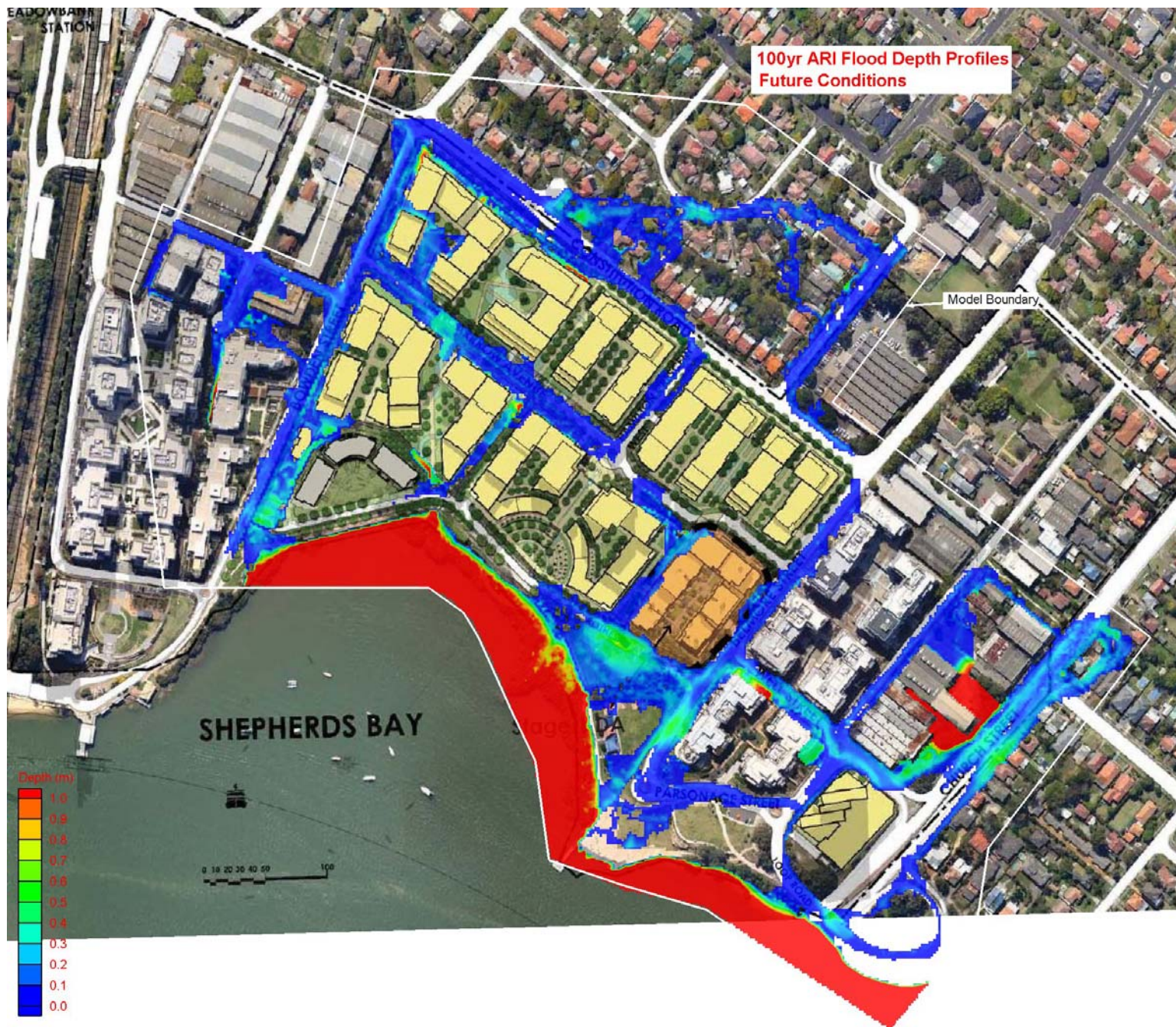
Figure 17 100 yr ARI Flood Levels – Future Conditions
