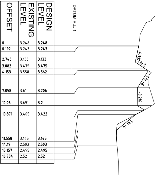
TYPICAL CROSS SECTION 4
