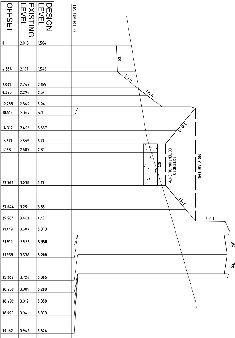
TYPICAL CROSS SECTION 7
