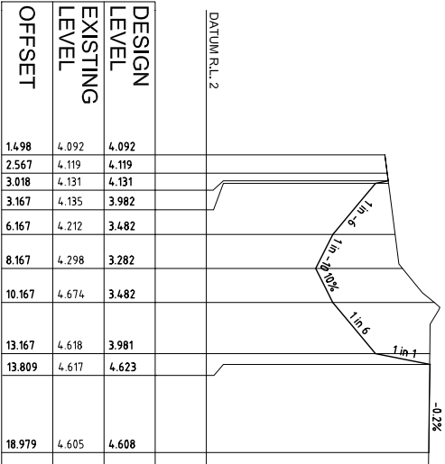
TYPICAL CROSS SECTION 3
