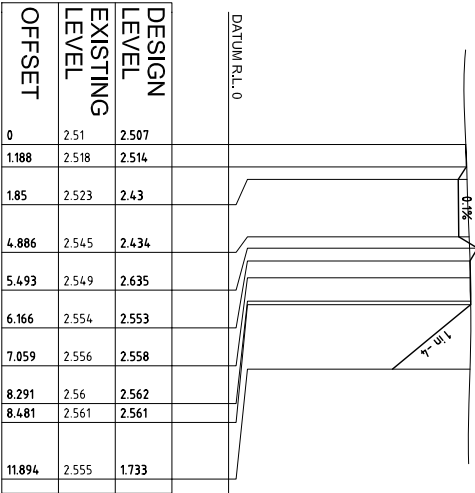
TYPICAL CROSS SECTION 5
