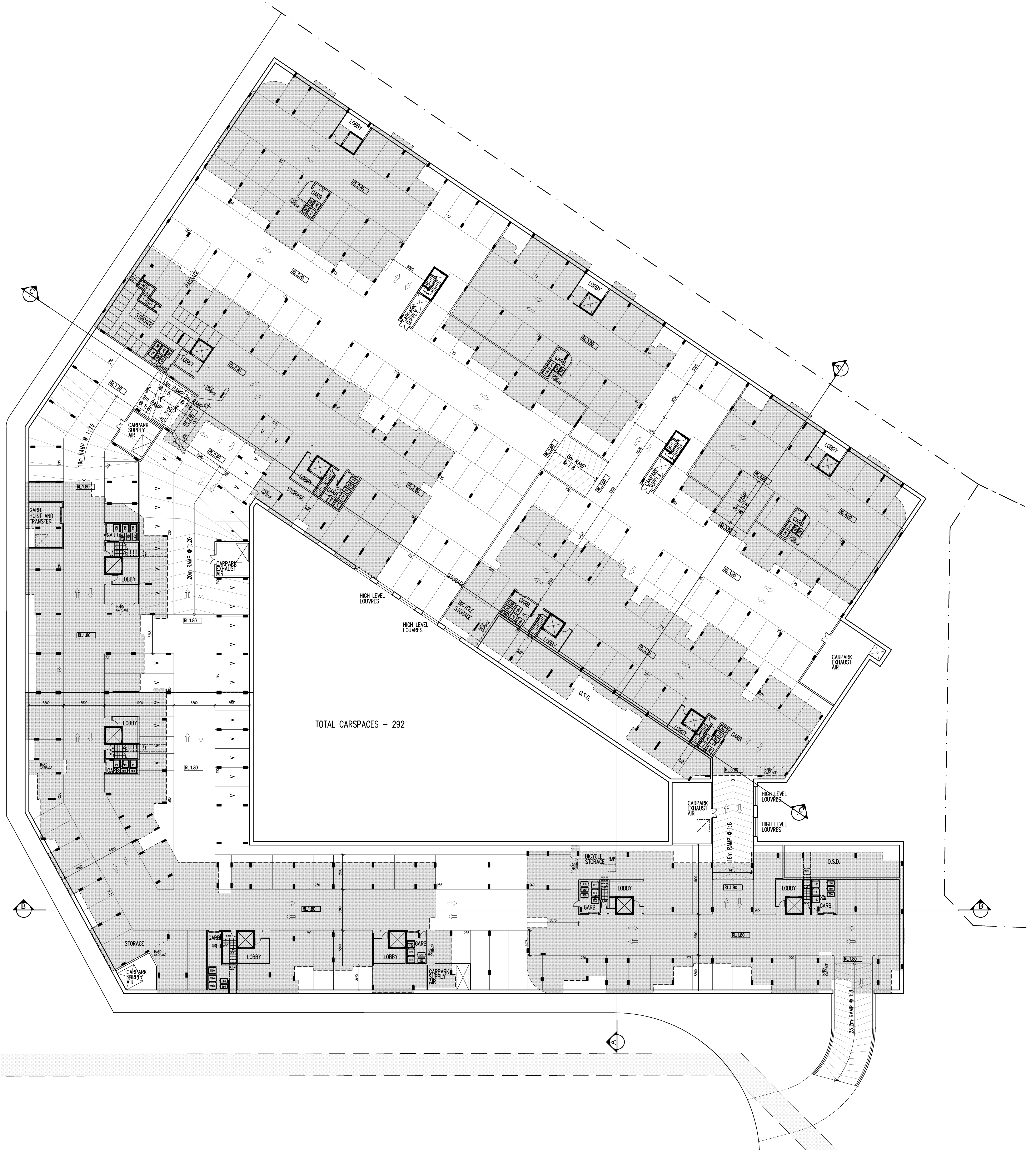
CARPARK LEVEL 2
