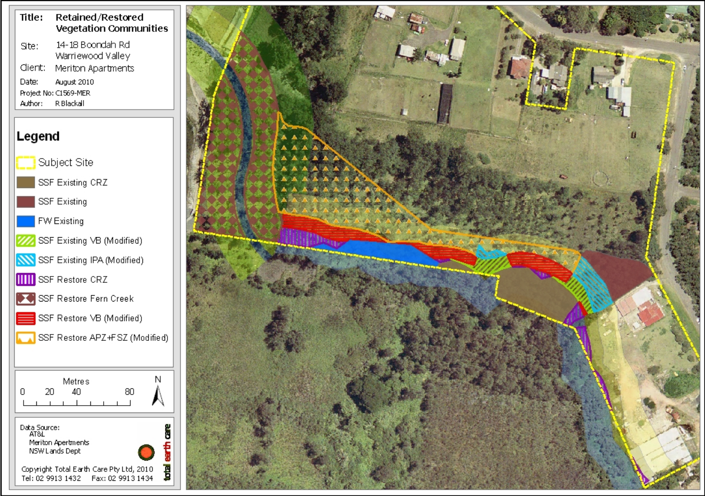
Figure 9: Vegetation management within riparian zones, retained SSF, APZ, Fern Creek and Flood Storage areas
