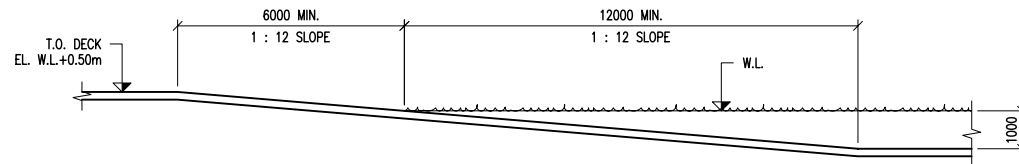
3 BEACH ENTRY SECTION 1 : 100
