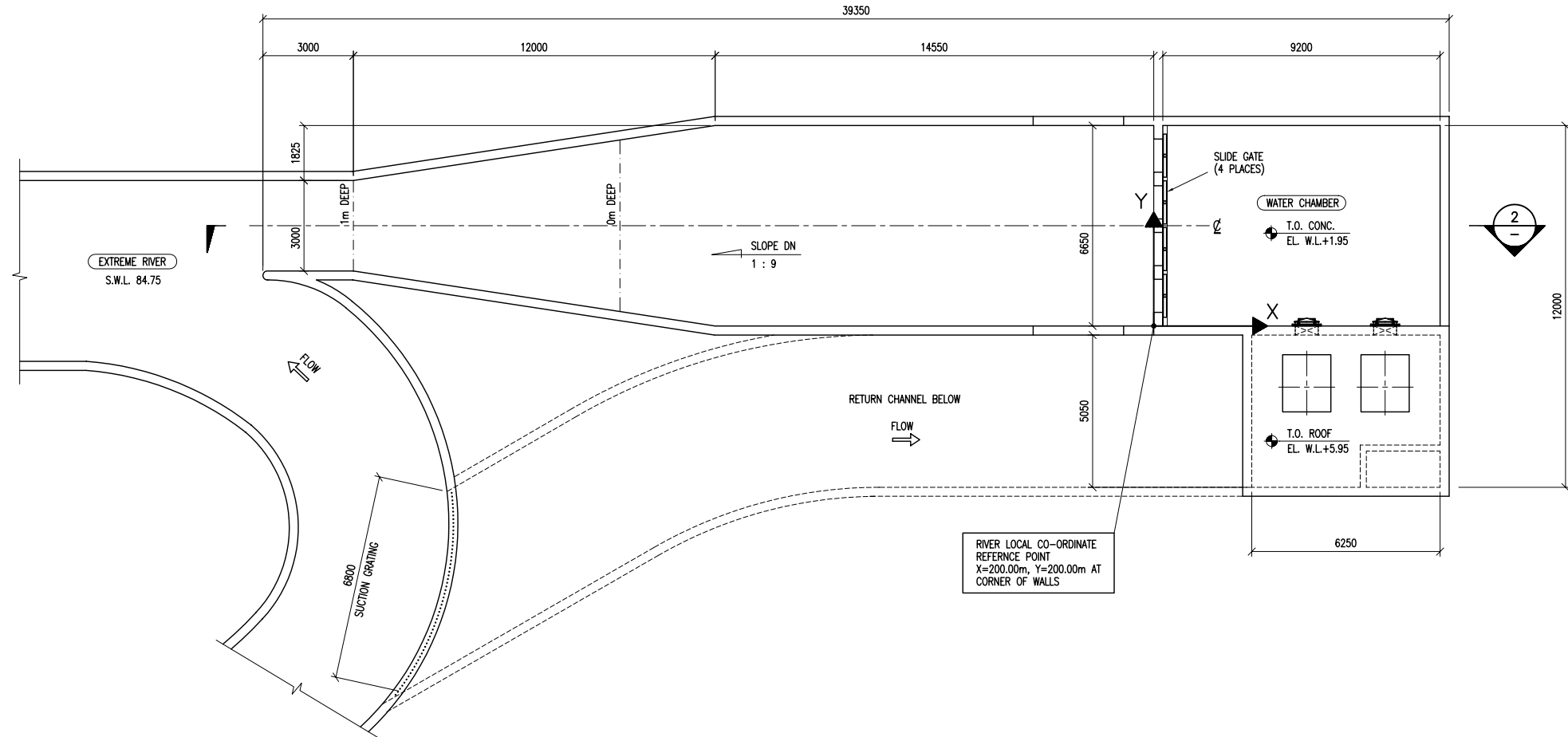
1 WAVE GENERATOR AREA PLAN 1 : 100
