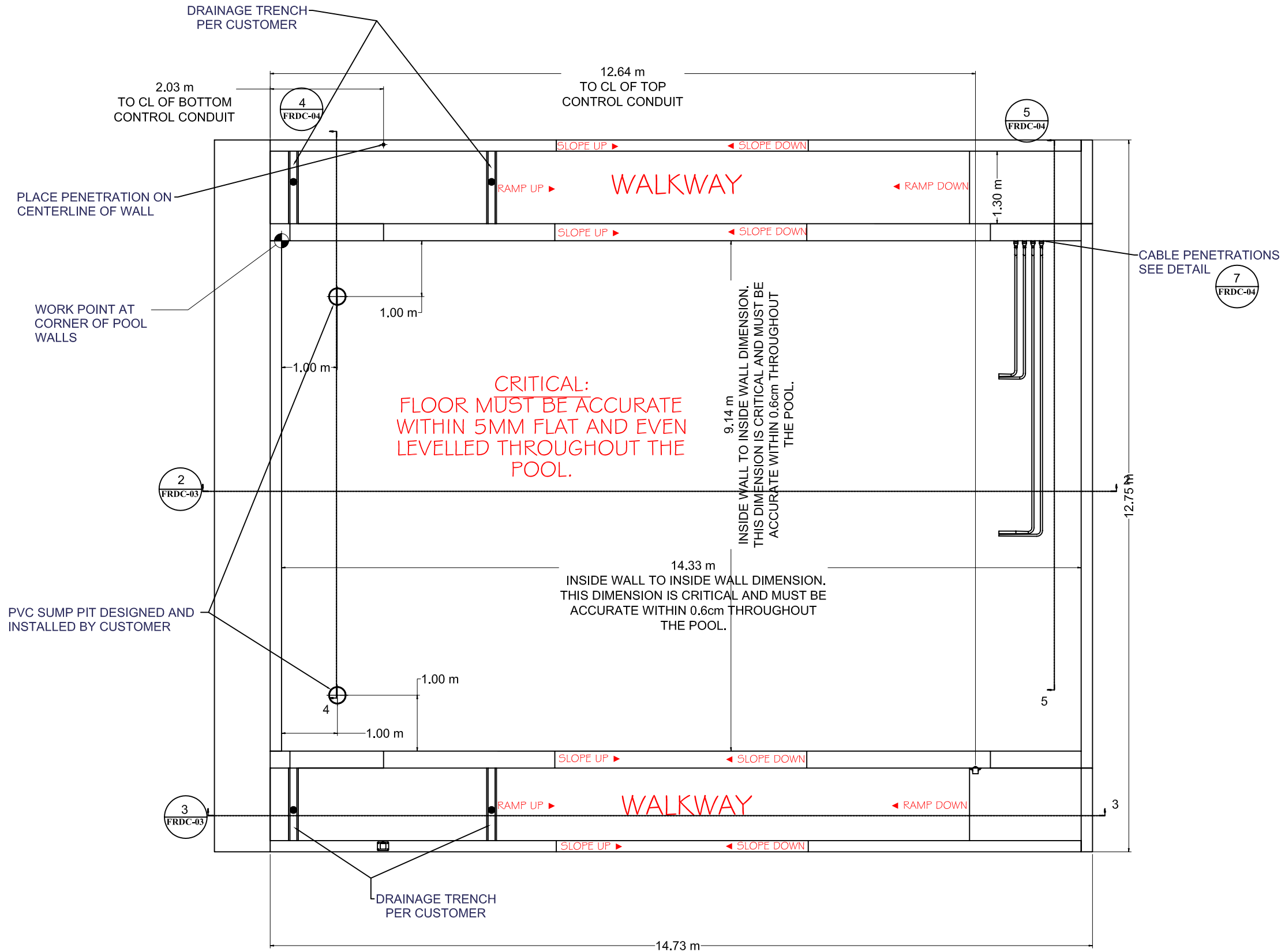
① PLAN VIEW FLOWRIDER DOUBLE WITH TWO WALKWAYS SHOWN
