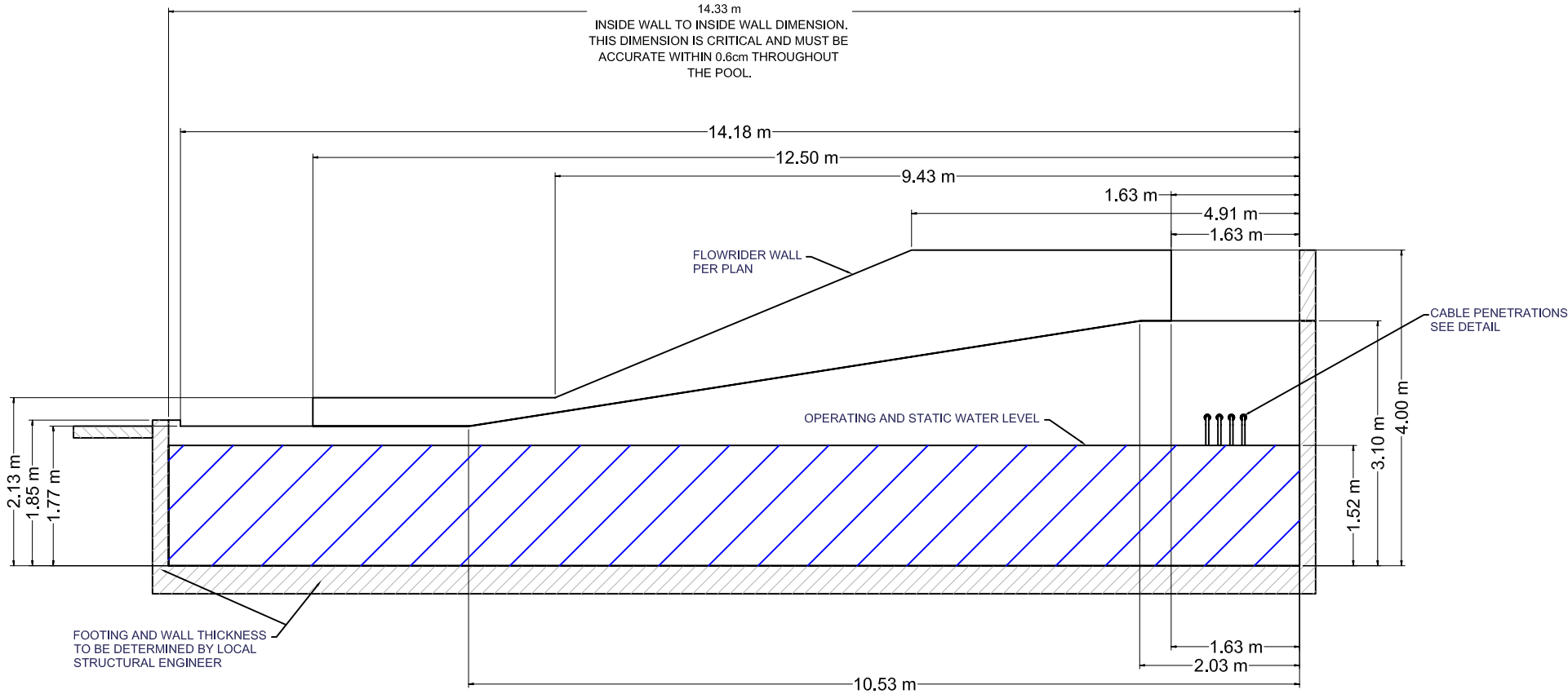
2 SECTION VIEW FLOWRIDER BASIN
