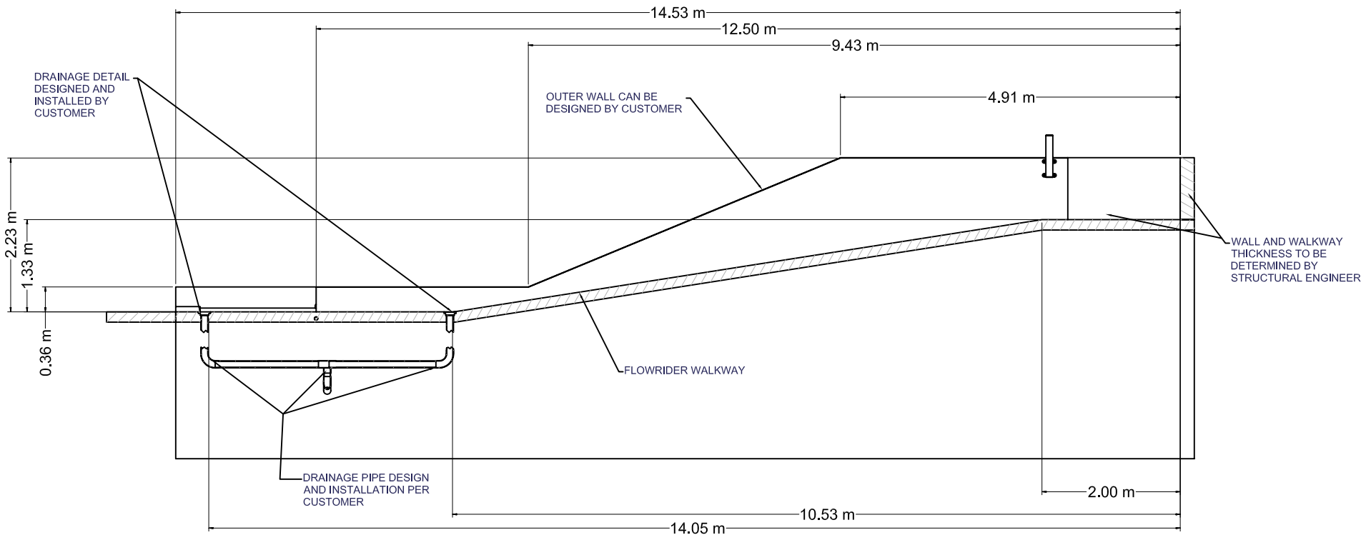
3 SECTION VIEW FLOWRIDER WALKWAY
