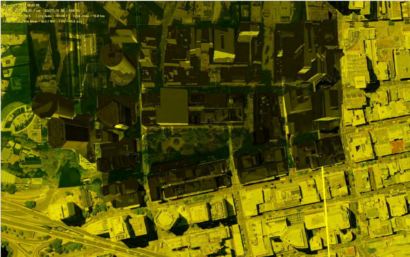
18:00:00 MARCH 22, 2010 SHADOW ANALYSIS FOLLOWING COMPLETION OF PROPOSED CITY ONE PROJECT
