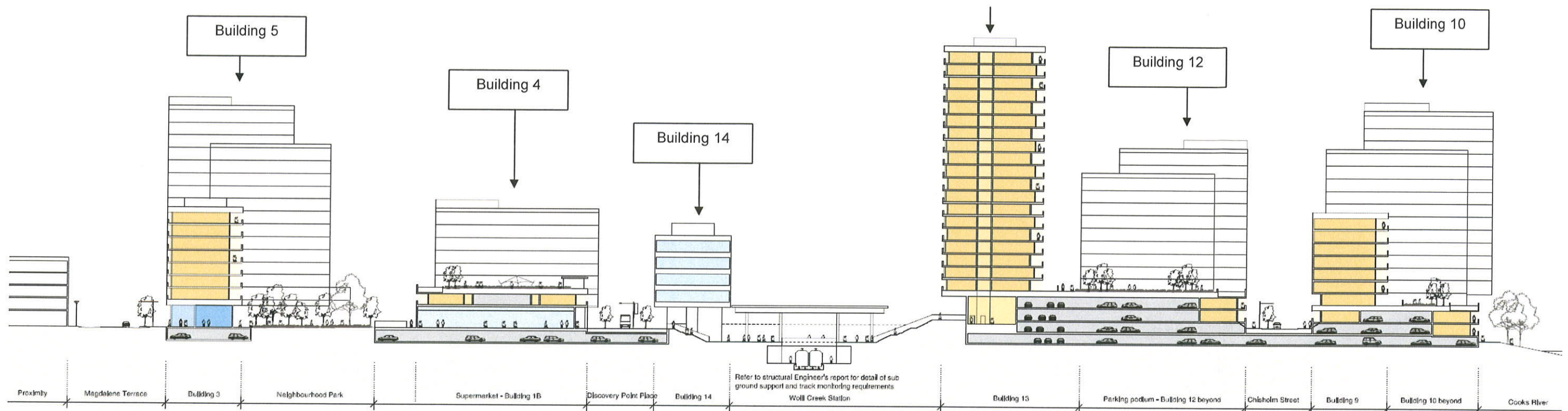
Figure 5: Indicative cross section design illustrating the mixture of residential (tan) and non-residential floor space (blue) across the site and parking areas (above and below ground), as contained in the PPR
