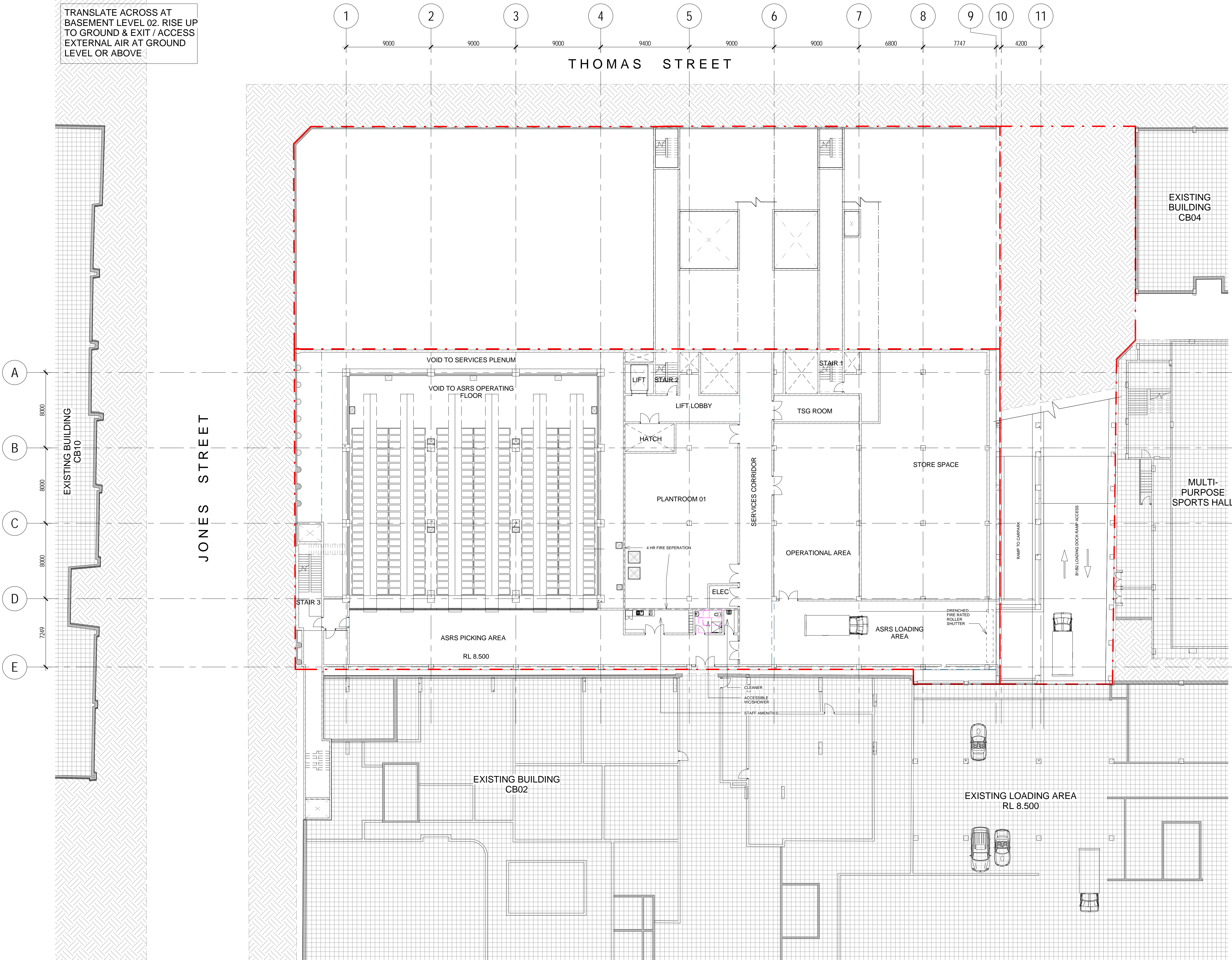
LEVEL 02 (RL 8.500) - EGRESS & SERVICE RISERS TRANSLATE AWAY FROM ALUMNI GREEN 1 : 200 (DIAGRAMMATIC ARRANGEMENT ONLY SUBJECT TO CHANGE WITH FINAL DESIGN)
