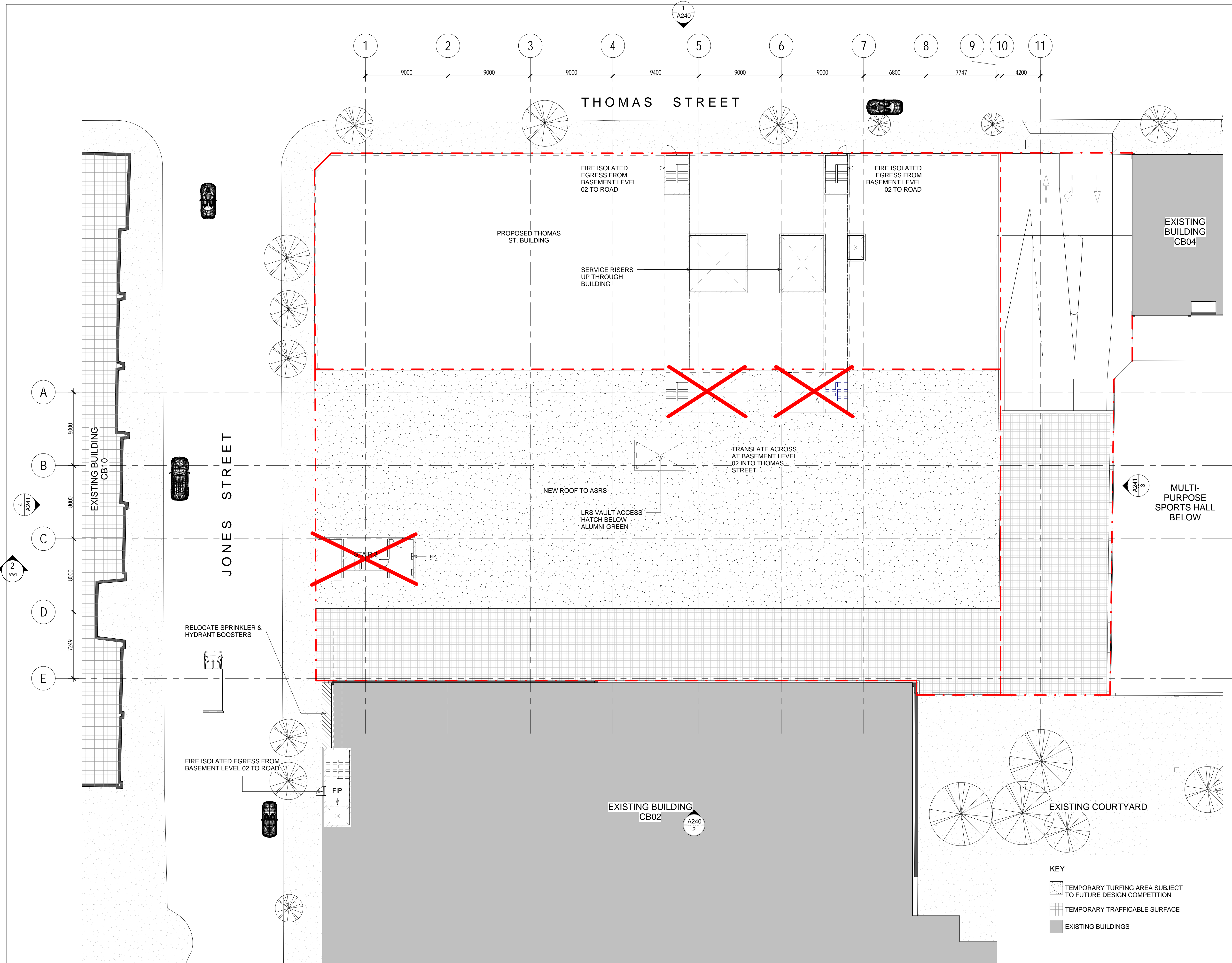
LEVEL 03 (RL 14.100) - EGRESS & SERVICE RISERS TRANSLATE AWAY FROM ALUMNI GREEN (DIAGRAMMATIC ARRANGEMENT ONLY SUBJECT TO CHANGE WITH FINAL DESIGN)
