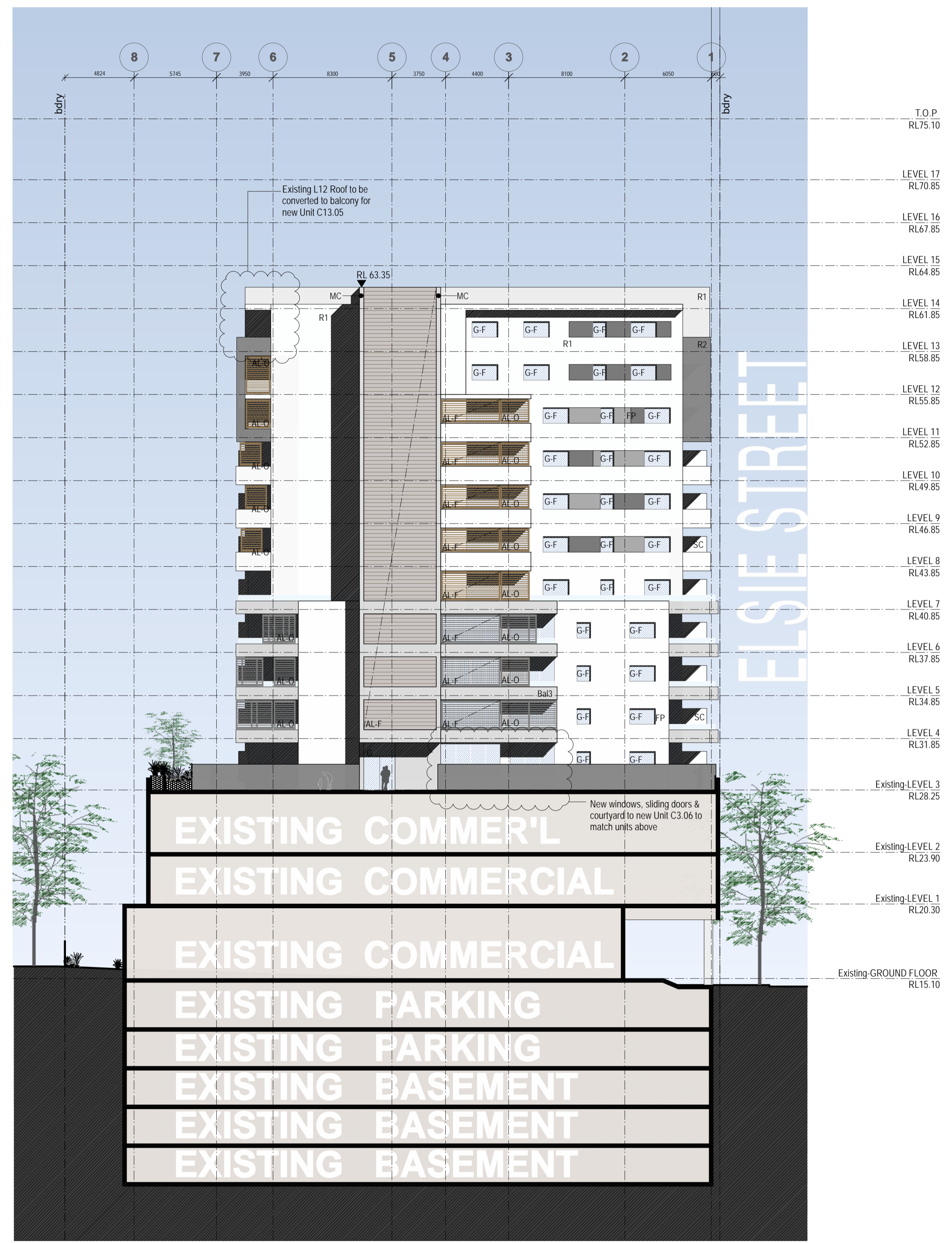
SOUTH ELEVATION - TOWER C
