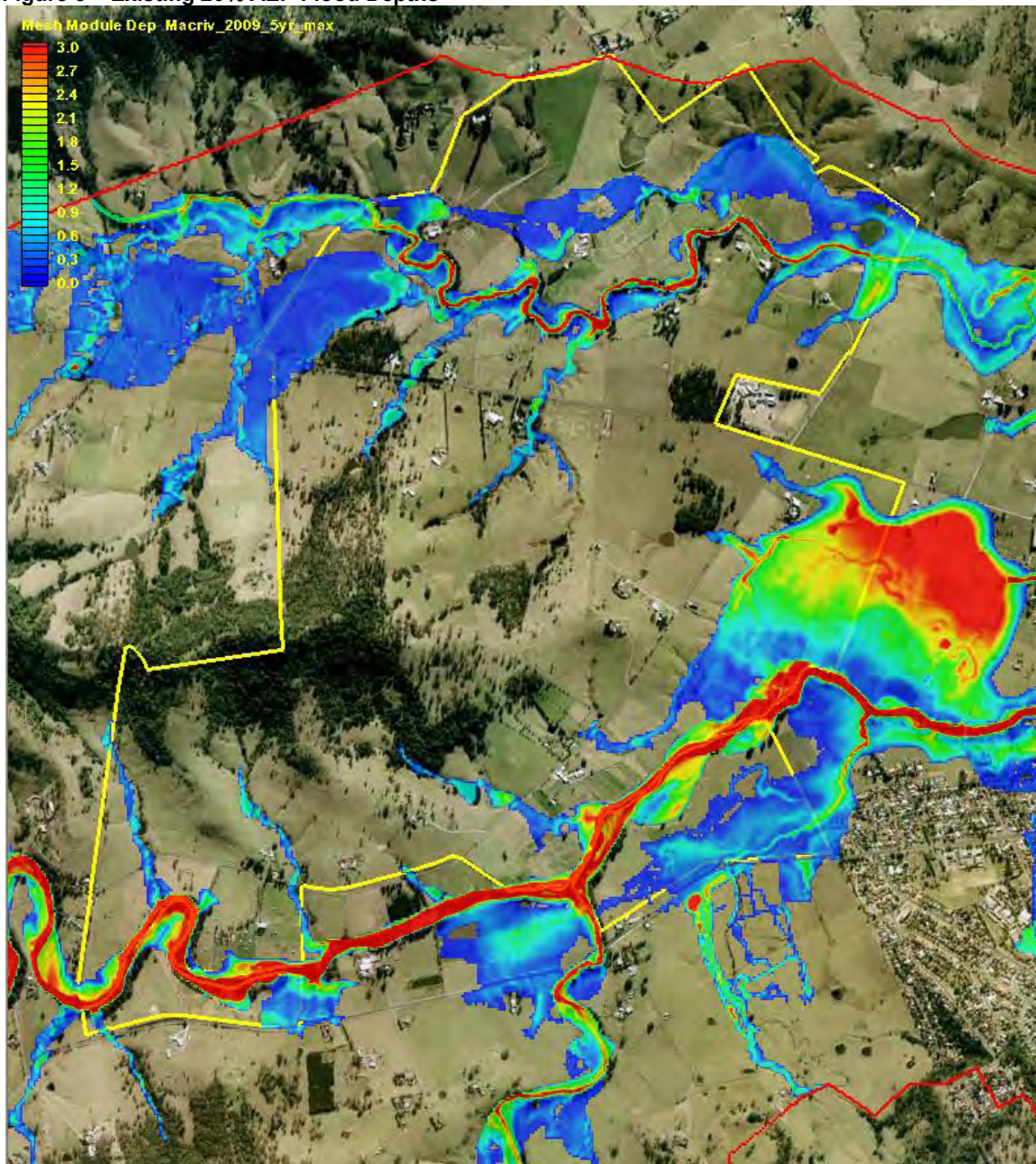
Figure 3 – Existing 20% AEP Flood Depths
