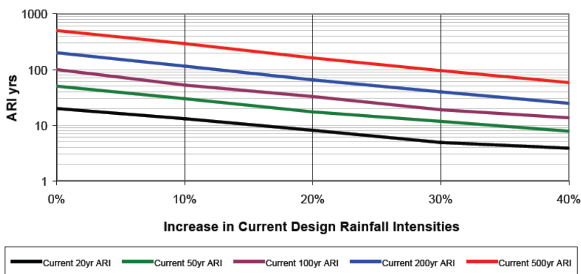
Figure 9 – Indicative Changes in Design ARI as Rainfall Intensity Increases
