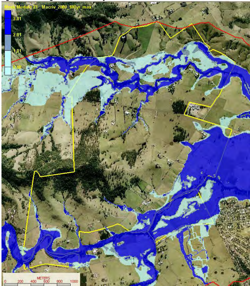
Figure 6 – Existing 1% Provisional Hydraulic Hazard
