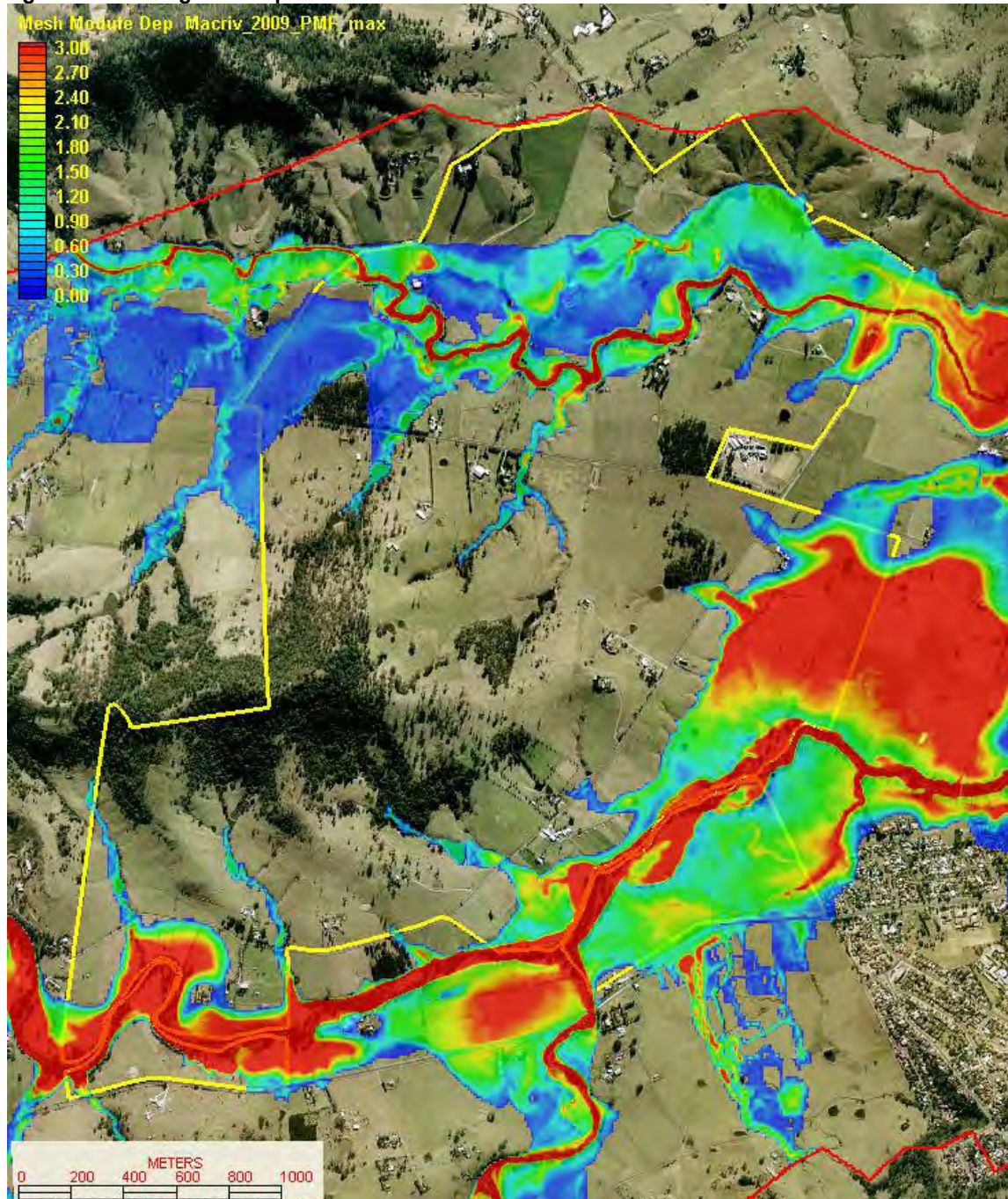
Figure 5 – Existing PMF Depths
