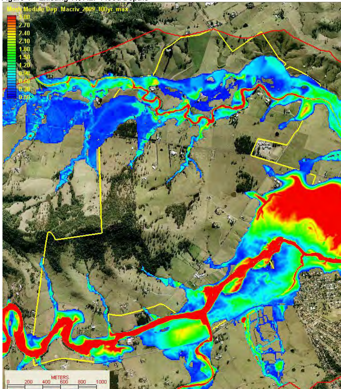
Figure 4 – Existing 1% AEP Flood Depths
