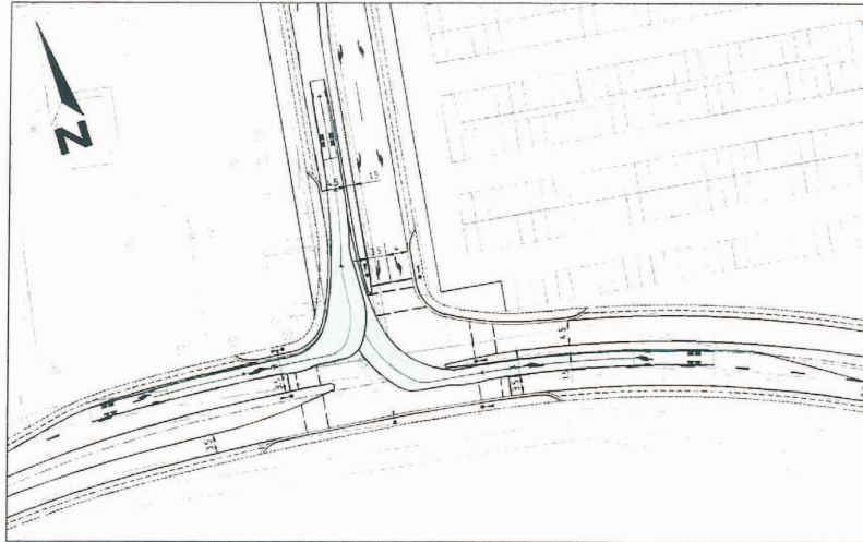
DESIGN VEHICLE 14.5M RIGID BUS TURN A AND C
