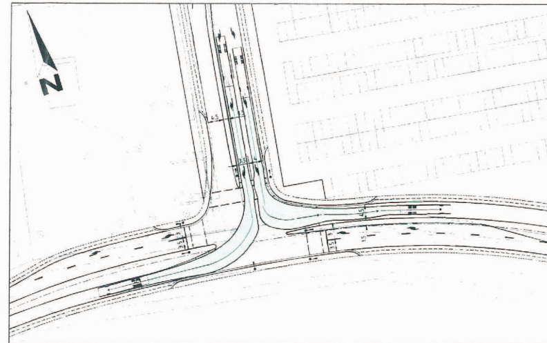
DESIGN VEHICLE 14.5M RIGID BUS TURN B AND D
