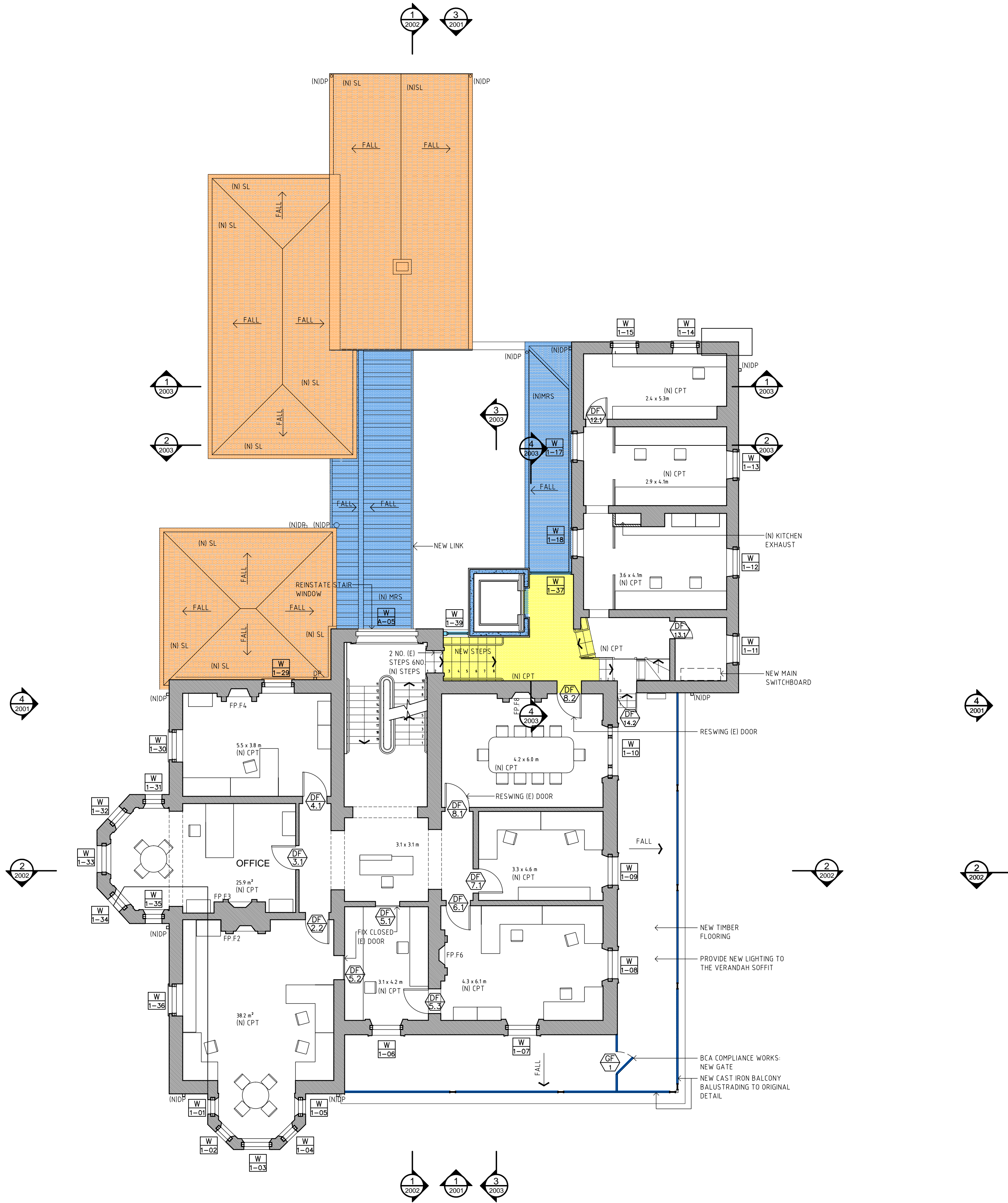
01 PROPOSED FIRST FLOOR PLAN 1:100
