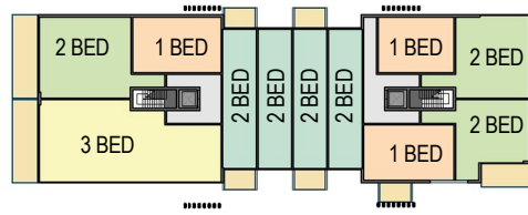
1 BLOCK D-E LEVEL 1 1 : 1000
