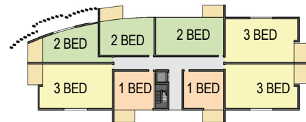
8 BLOCK H TYPICAL FLOOR PLAN 1 : 1000
