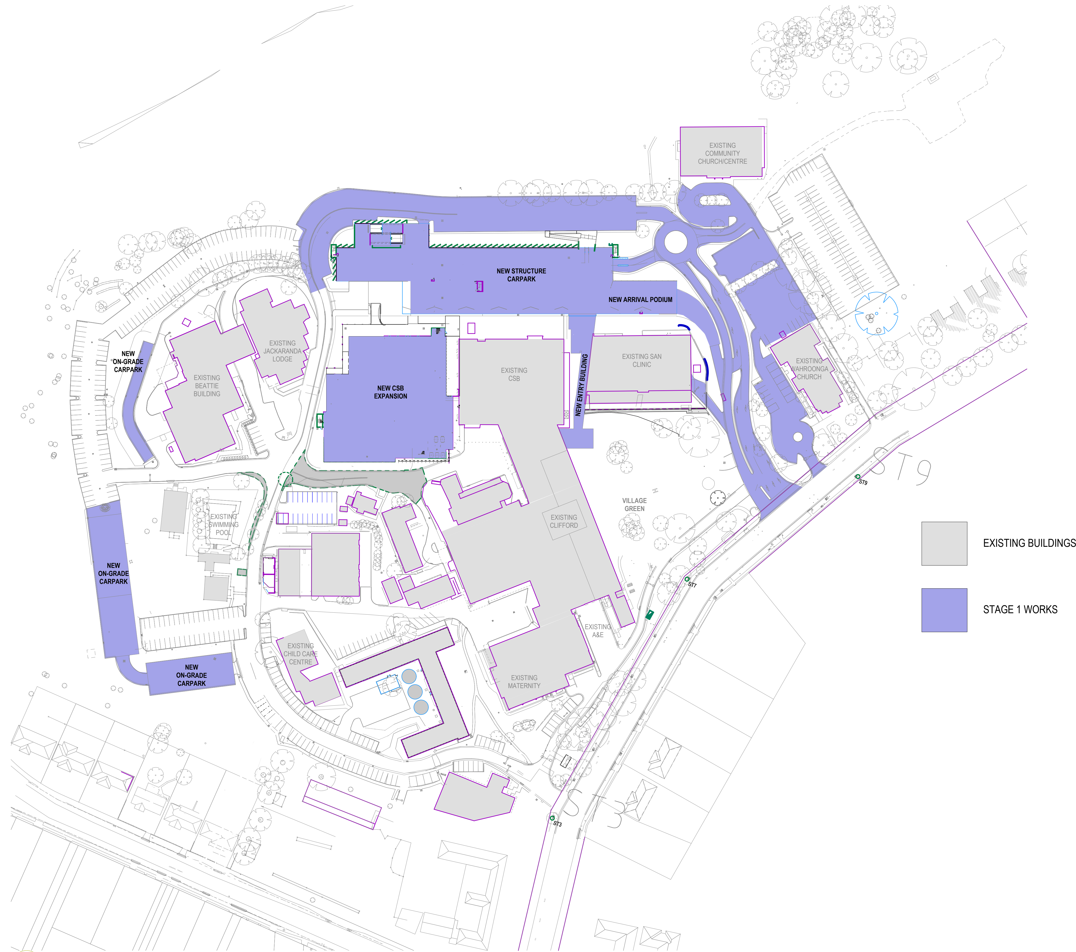
1 Proposed MasterPlan Stage 1 SCALE 1:1000
