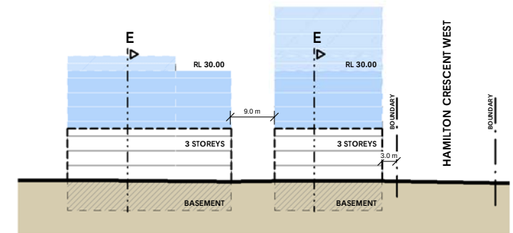
4. Constitution Road EA004-A 1 : 500
