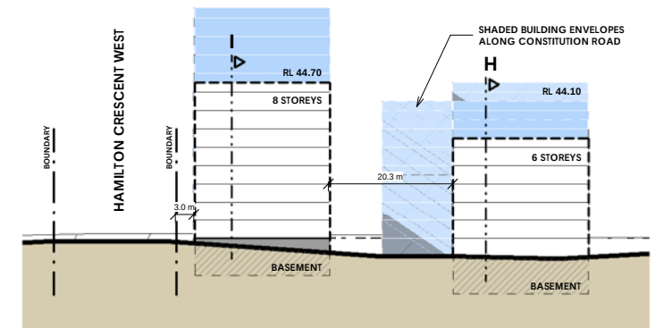
4. Nancarrow Ave - NORTH EA004-A 1 : 500
