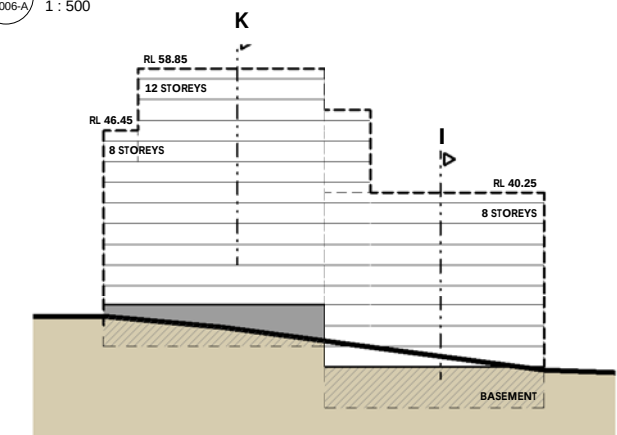
6. Nancarrow Avenue - South 1 : 500
