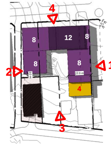
6. Building Envelope Plan 1 : 1000
