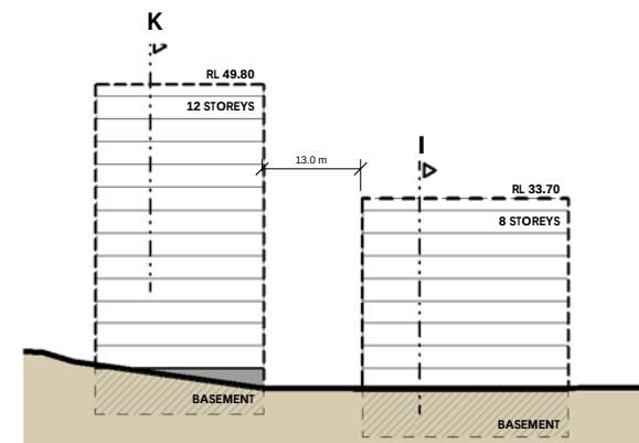
4 7. Nancarrow Avenue - South EA007-A 1 : 500
