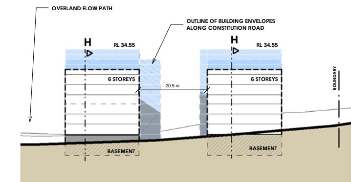
3 8. Street elevation - Nancarrow Ave - NORTH EA008-A 1 : 500
