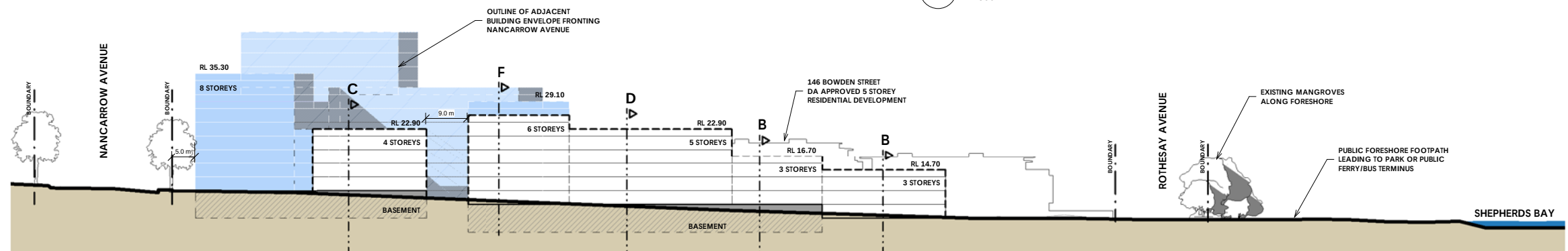
9. Bowden Street 1 : 500
