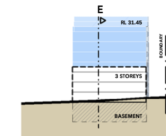
4 10. Constitution Road 1 : 500
