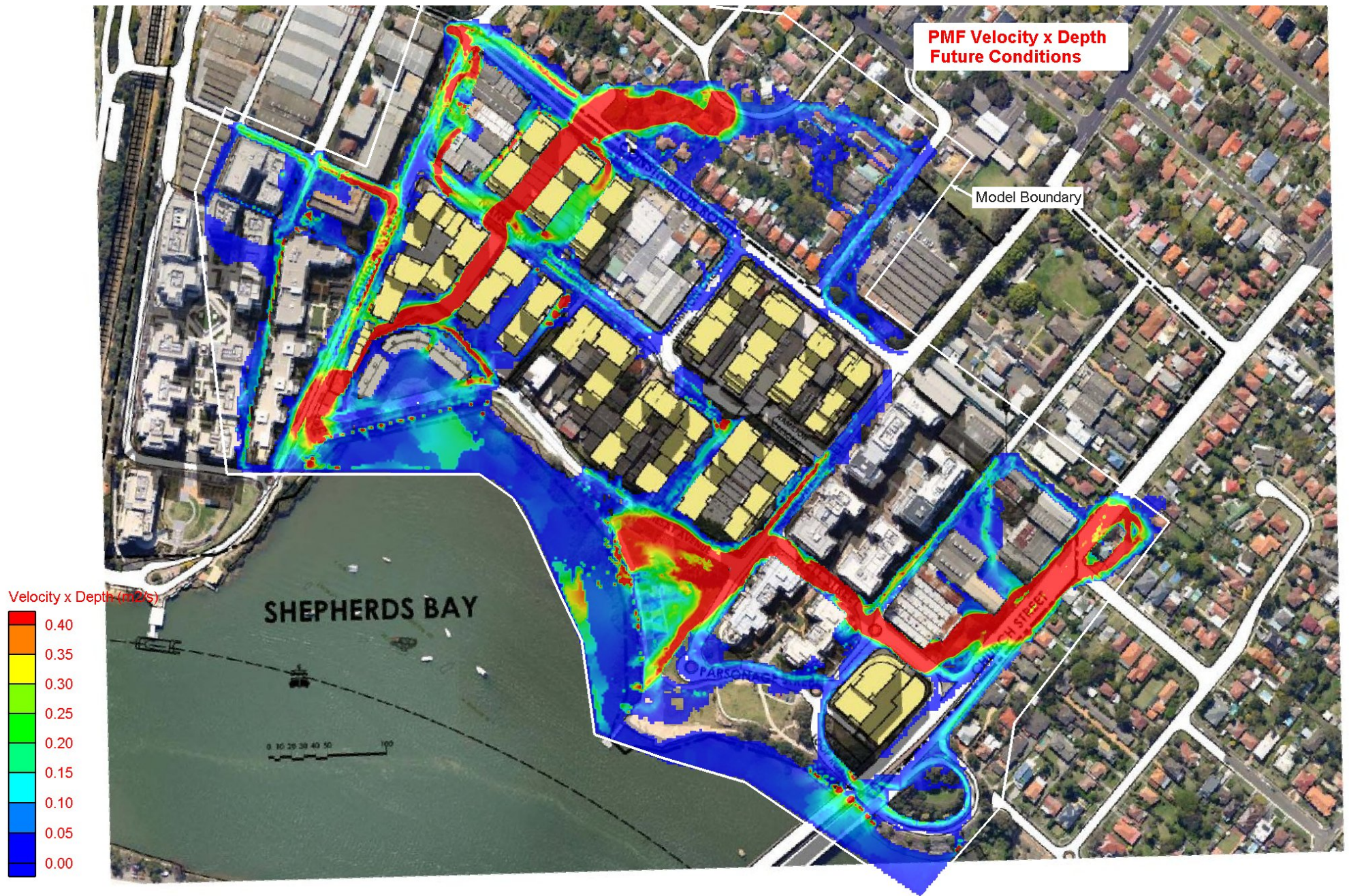
Figure 23 PMF Flood Velocity x Depth – Future Conditions
