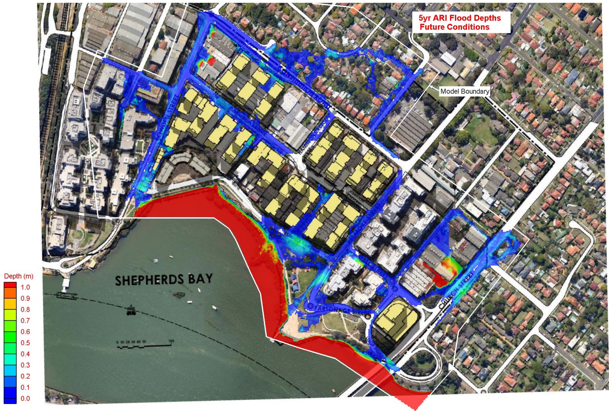
Figure 13 5 yr ARI Flood Levels – Future Conditions
