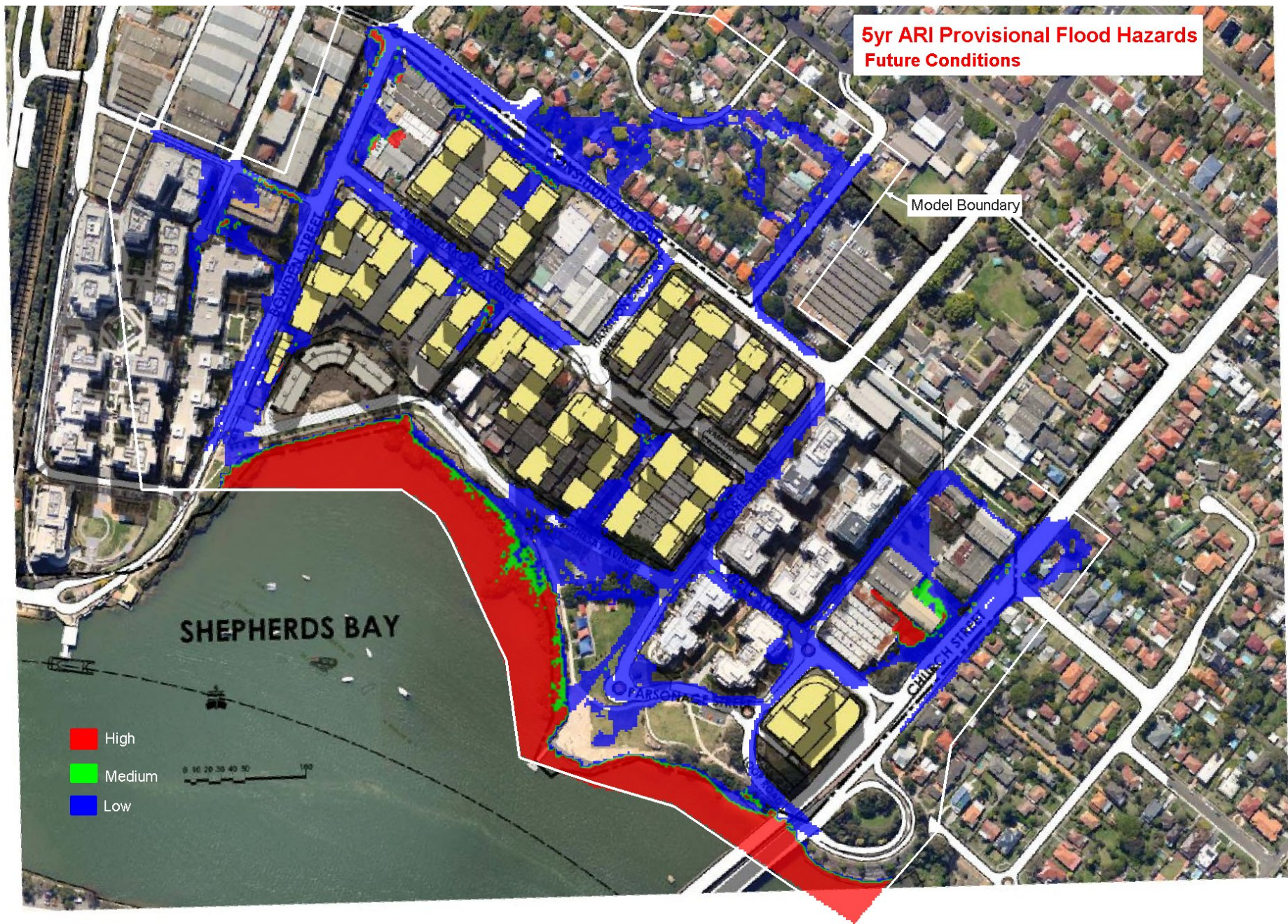
Figure 16 5 yr ARI Flood Hazard – Future Conditions
