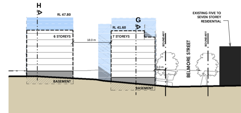
2. Nancarrow Ave - NORTH EA002-A 1 : 500
