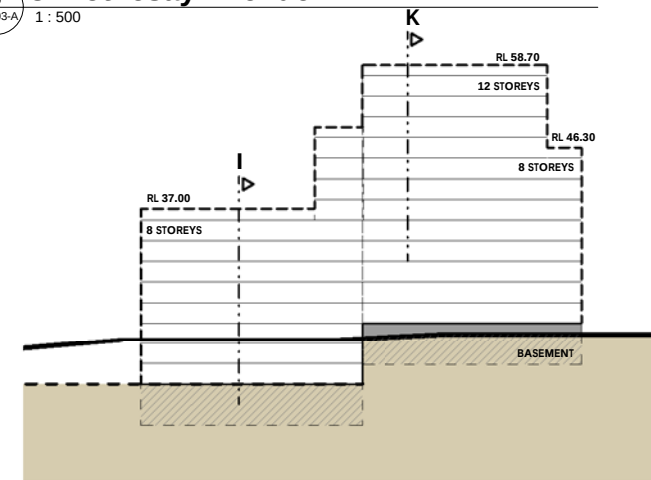
3. Nancarrow Avenue - South EA003-A 1: 500
