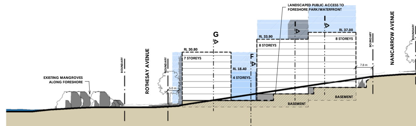
3. Elevation 2 EA003-A 1: 500
