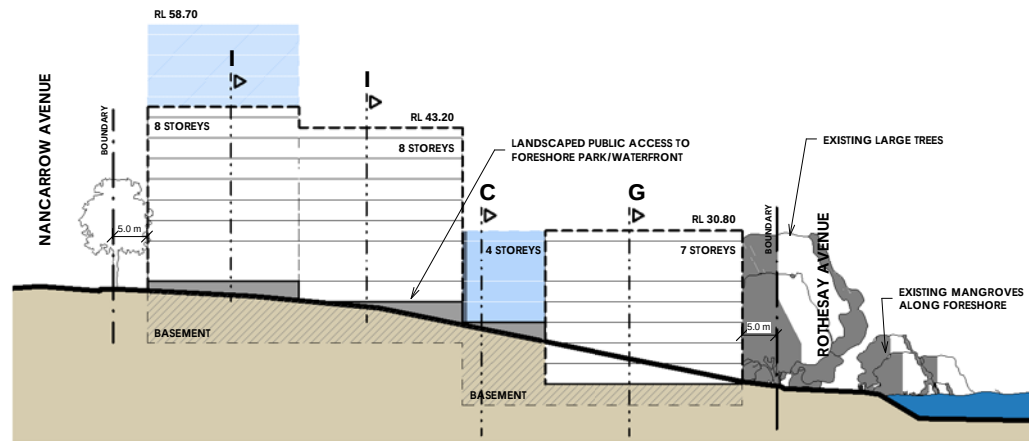
3. Elevation 1 EA003-A 1: 500
