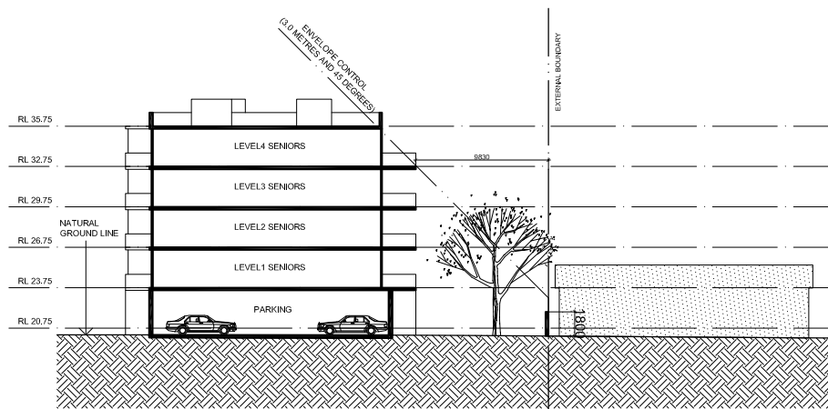
SECTION CC LOT 31 SENIORS LIVING COMPLEX
