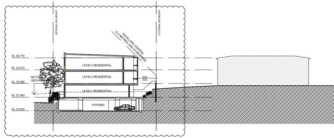
SECTION AA LOT 21 RESIDENTIAL BUILDING
